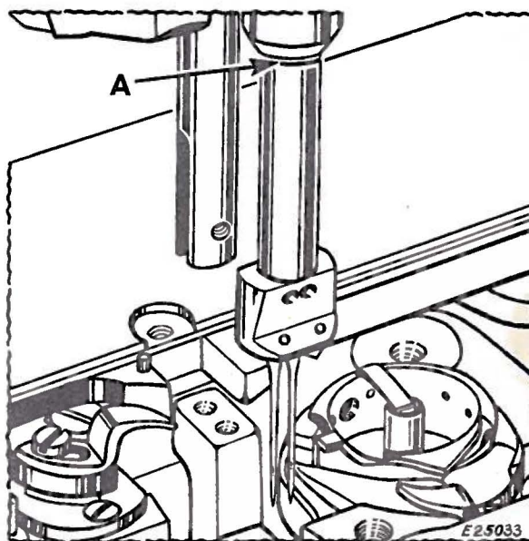
Fig. 16. Height Adjustment of Sewing Hook
