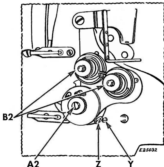
Fig. 15. Adjustment of Thread Controller
